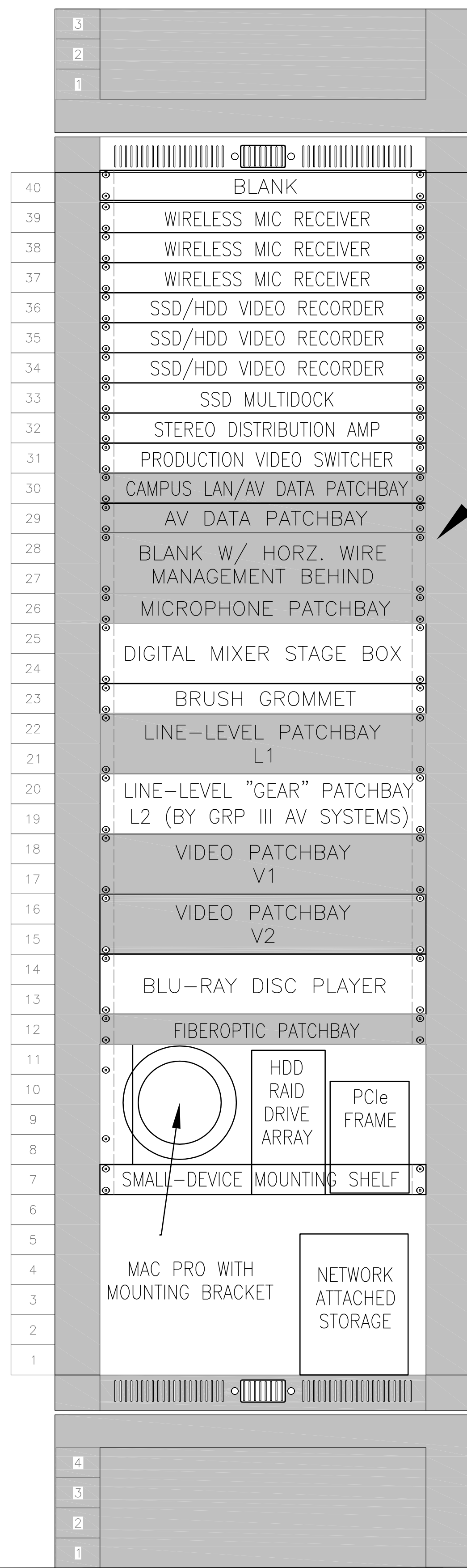
RACK TV STUDIO - MAIN RACK 11 LOCATION: WALL MOUNT IN CONTROL ROOM
