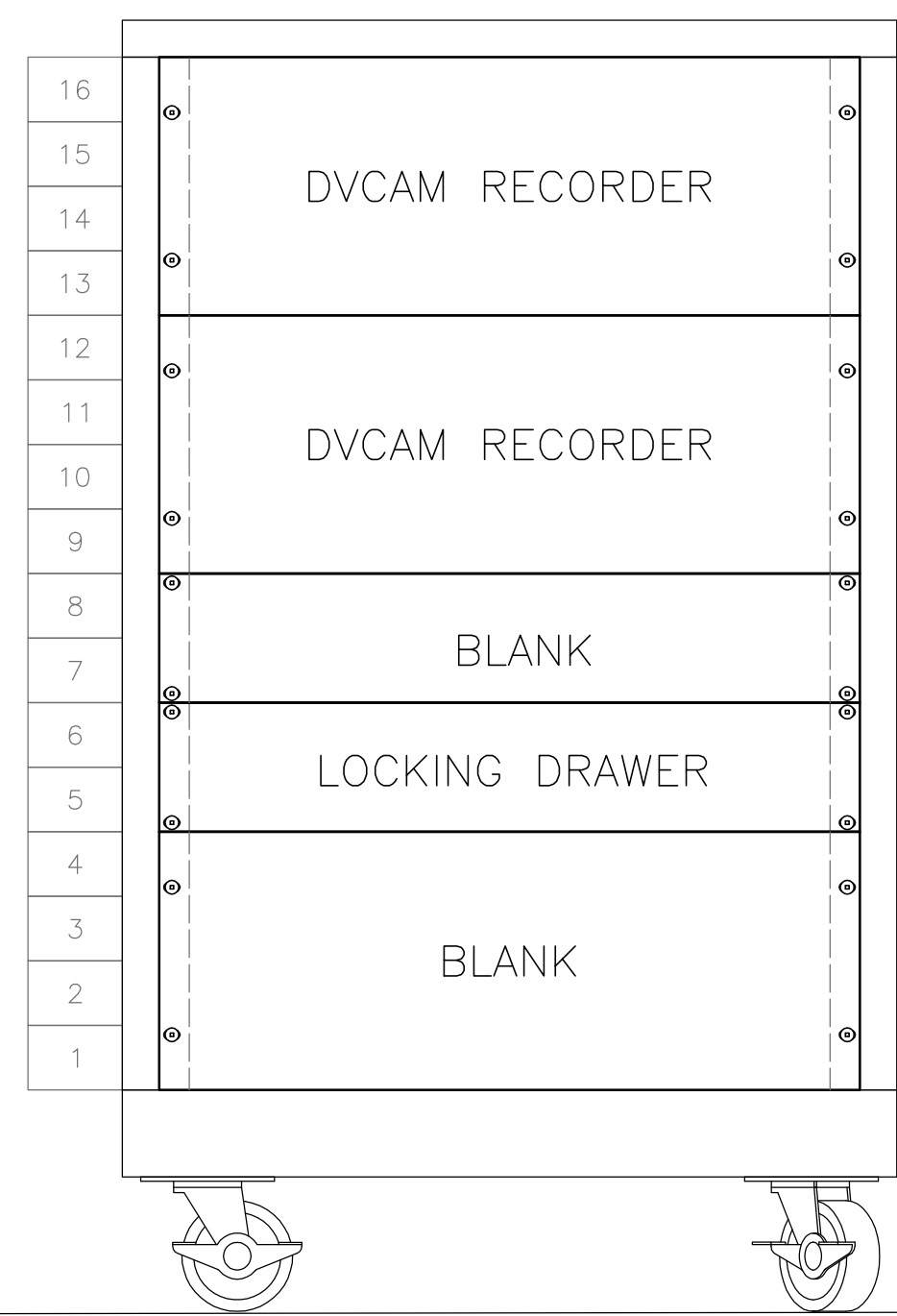
RACK ANCILLARY MOBILE RACK 12 LOCATION: PARK IN TV STUDIO CONTROL BOOTH
