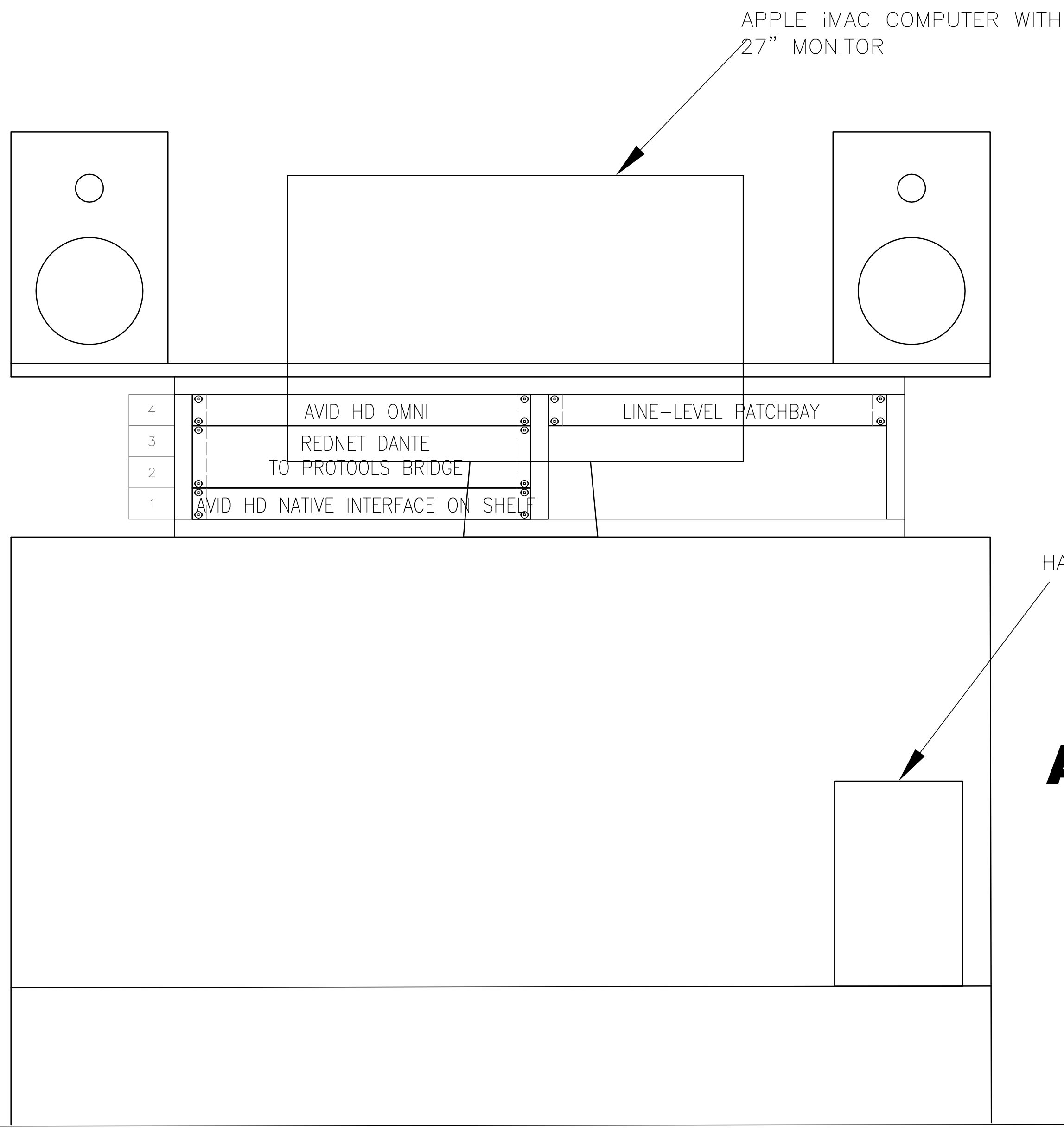
RACK SOUND EDIT ROOM BRIDGE RACKS 13 LOCATION: SOUND EDIT ROOM
