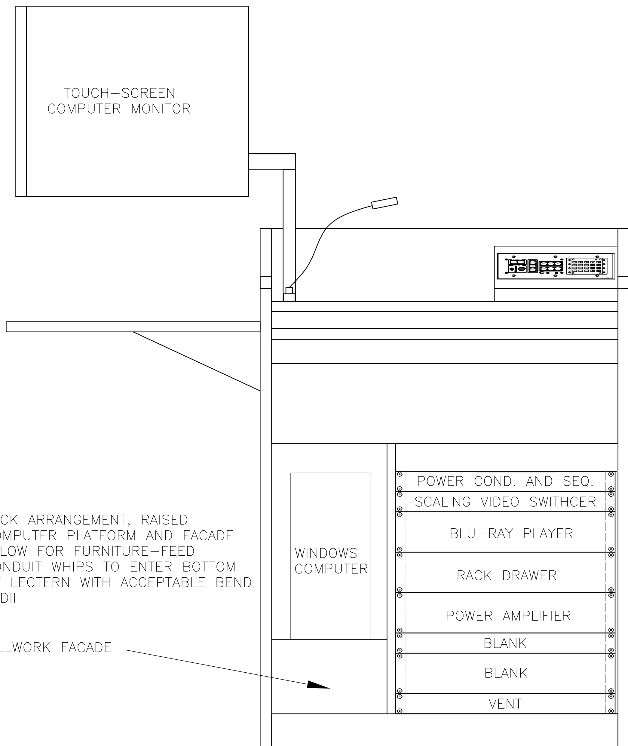
RACK 7 CLASSROOM - FIXED LECTERN LOCATION: Rms. 139, 140, 141, 142, 144, 154, 233, 234, 243, 244, 245, 246, 247, 252
