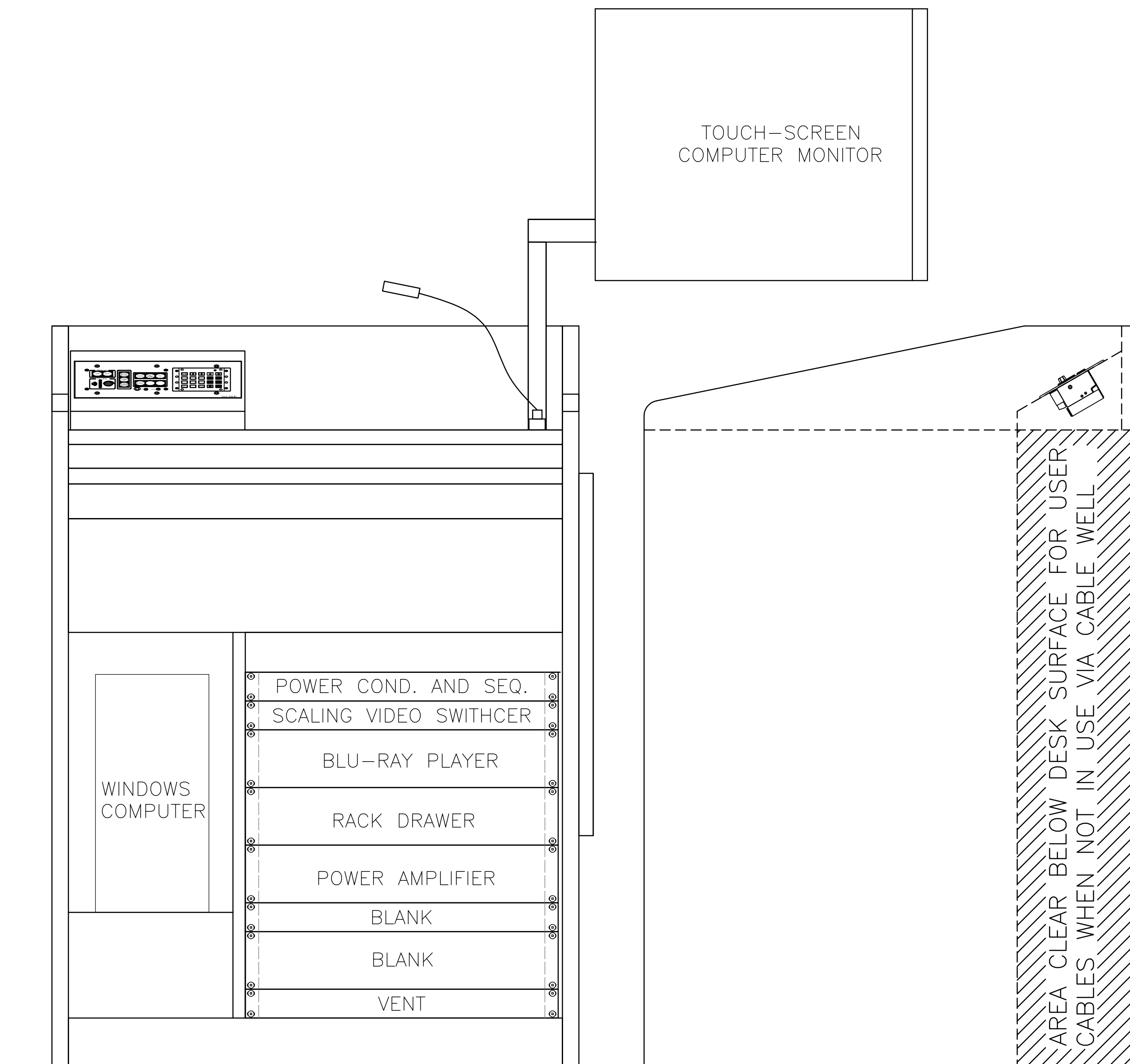
RACK 8 CLASSROOM - FIXED LECTERN RACK LOCATION: Rms. 143, 235, 253, 256
