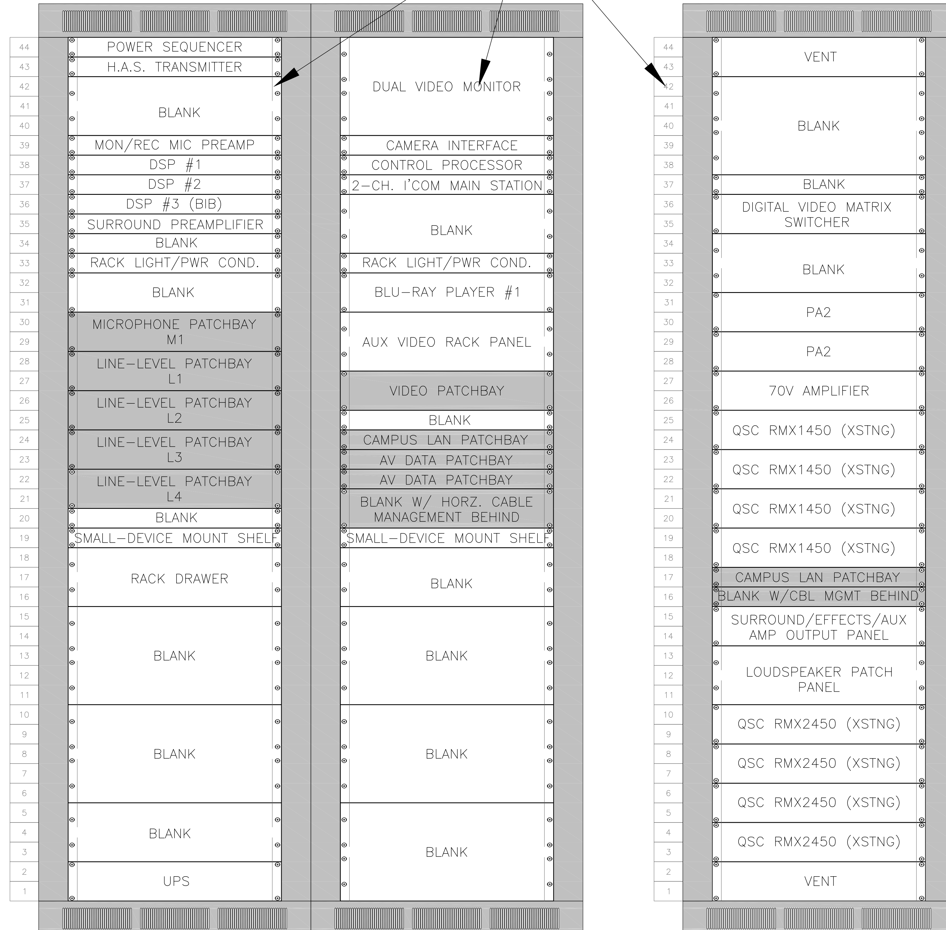
RACK 1 THEATER - PATCHING AND FRONT-END RACKS LOCATION: SOUND CONTROL BOOTH
