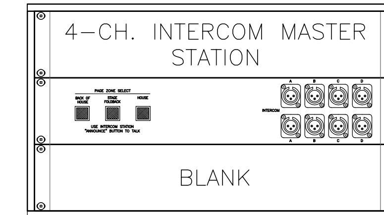
RACK 4 THEATER - STAGE MANAGER RACK LOCATION: PORTABLE
