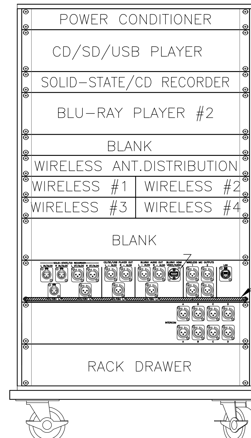
RACK 3 THEATER - MOBILE ANCILLARY RACK LOCATION: MOBILE
