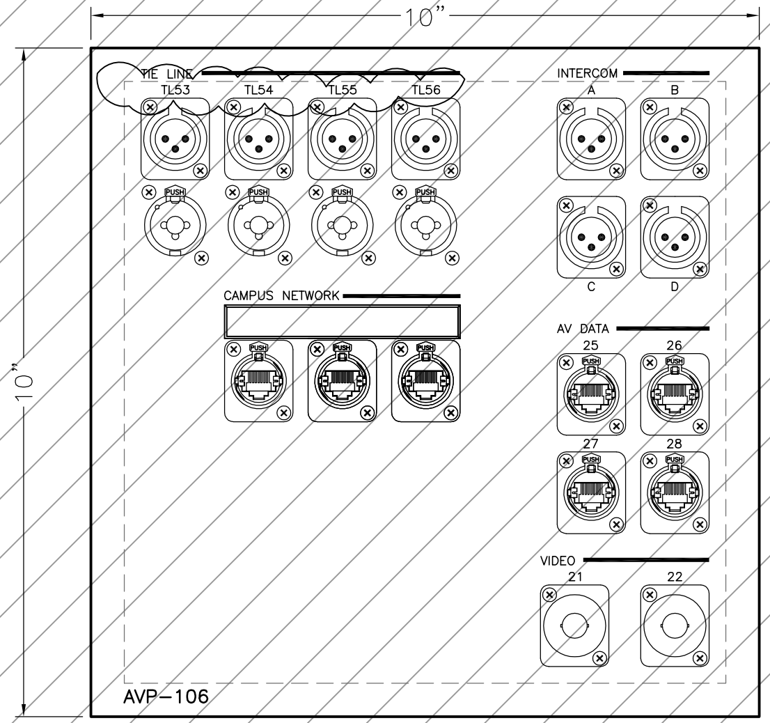
AVP-106 LIGHTING BOOTH SURFACE-MOUNT BOX
