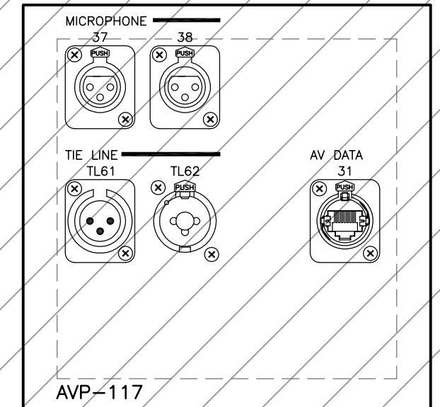
AVP-117 OVER STAGE; PIPE-GRID-MOUNT
