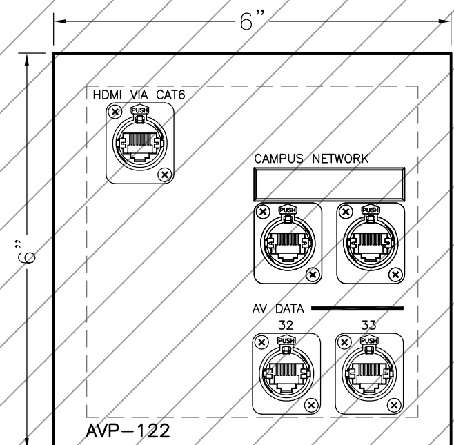
AVP-122 THEATER PROJECTION BOOTH SURFACE-MOUNT AT CEILING
