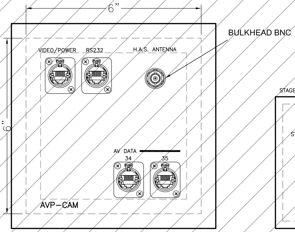
AVP-CAM THEATER REAR WALL FLUSH-MOUNT
