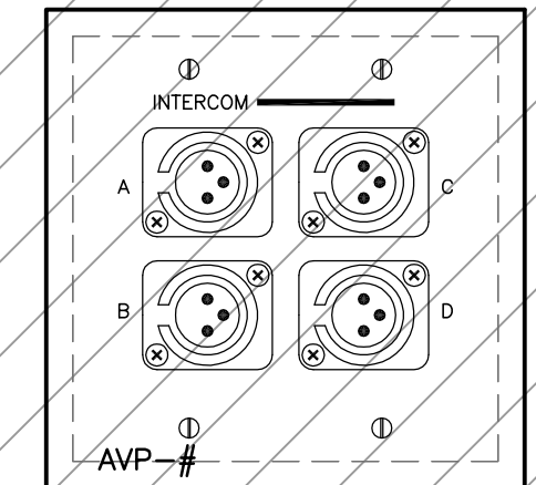
AVP-110, 112 INTERCOM; 2-GANG FLUSH-MOUNT
