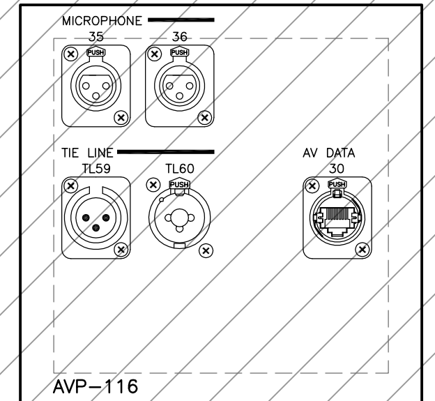
AVP-116 OVER STAGE; PIPE-GRID-MOUNT
