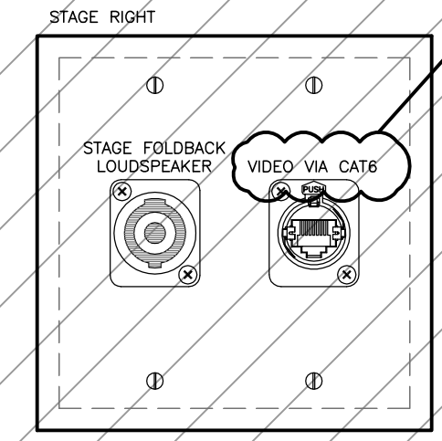
AVP-STGF THEATER - PROSC. WALL FLUSH-MOUNT
