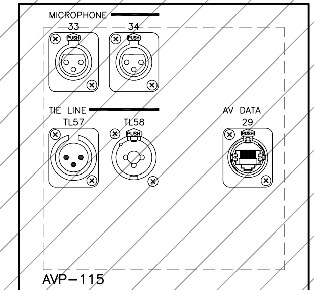
AVP-115 OVER STAGE; PIPE-GRID-MOUNT
