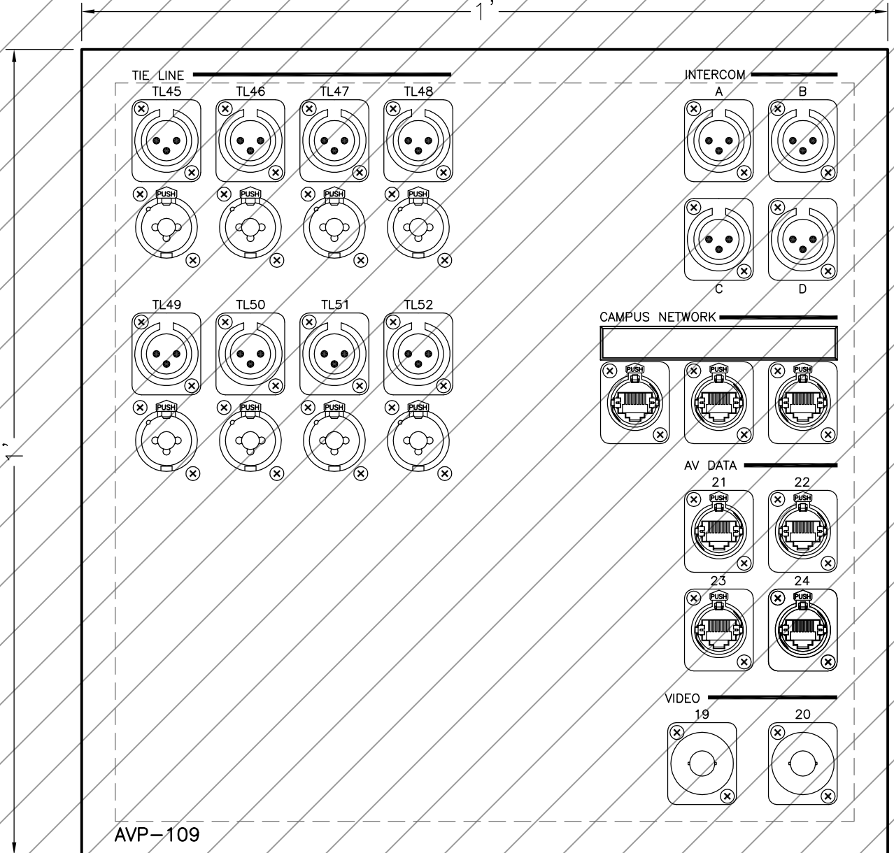
AVP-109 AT PROJECTION BOOTH SURFACE-MOUNT BOX
