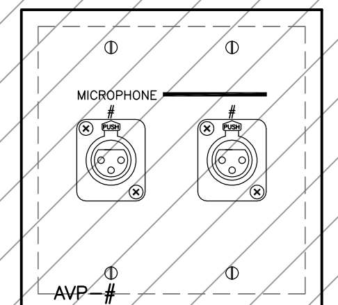
AVP-118 (MIC 39,40), AVP-119 (MIC 41,42), AVP-120 (MIC 43,44), AVP-121 (MIC 45, 46) MICROPHONES AT CEILING; 2-GANG FLUSH-MOUNT
