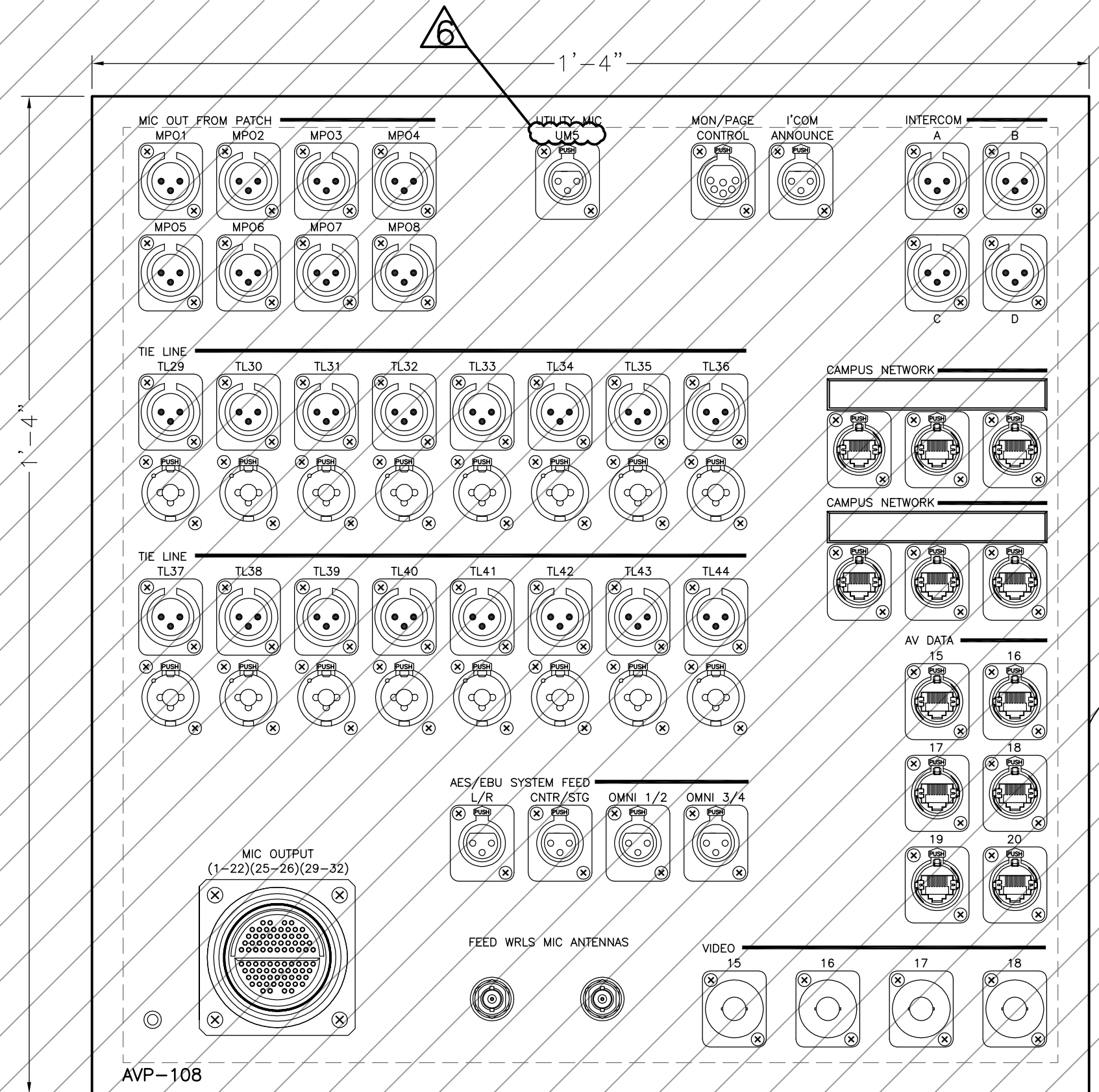
AVP-108 MIX POSITION AT CONTROL BOOTH SURFACE-MOUNT BOX
