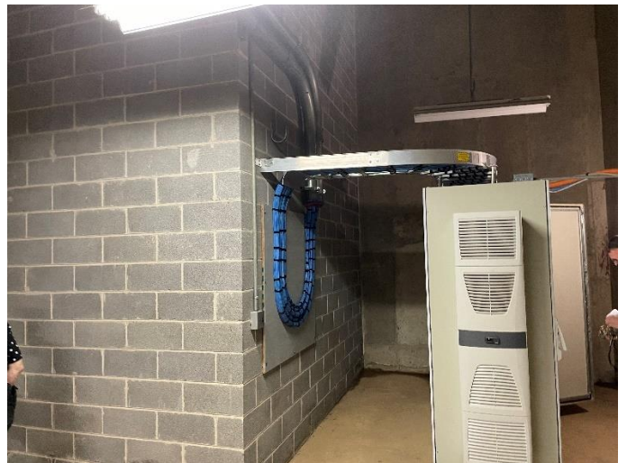
View of Telecom Cable Tray (South End)
