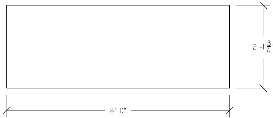
LID TYPE A 0'-0 1/2"=1'-0" CUT FROM 3/4" AC PLY
