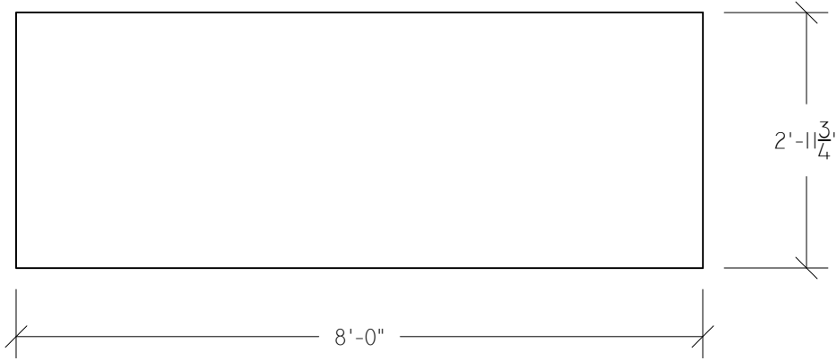
LID TYPE A 0'-0 1/2"=1'-0" CUT FROM 3/4" AC PLY (LIDS 1, 2, 4-6, 8-12)
