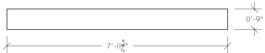
POOL EXTERIOR FASCIA TYPE C 0'-0 1/2"=1'-0" CUT FROM 1/4" AC PLY CUT 4
