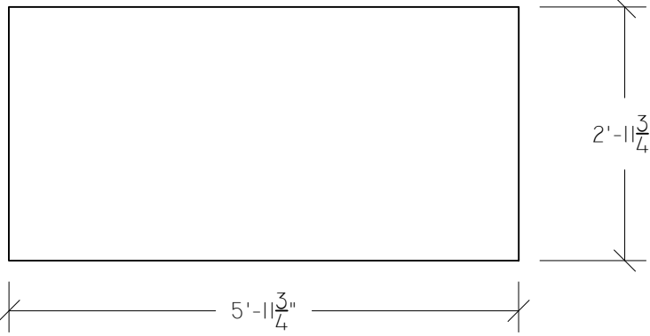
LID TYPE B 0'-0 1/2"=1'-0" CUT FROM 3/4" AC PLY (LIDS 3+7)
