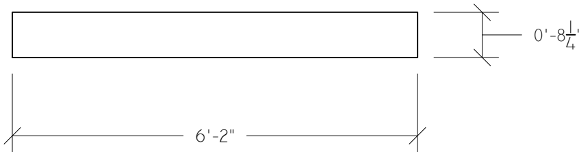
POOL INTERIOR FASCIA TYPE C 0'-0 1/2"=1'-0" CUT FROM 3/4" AC PLY CUT 4
