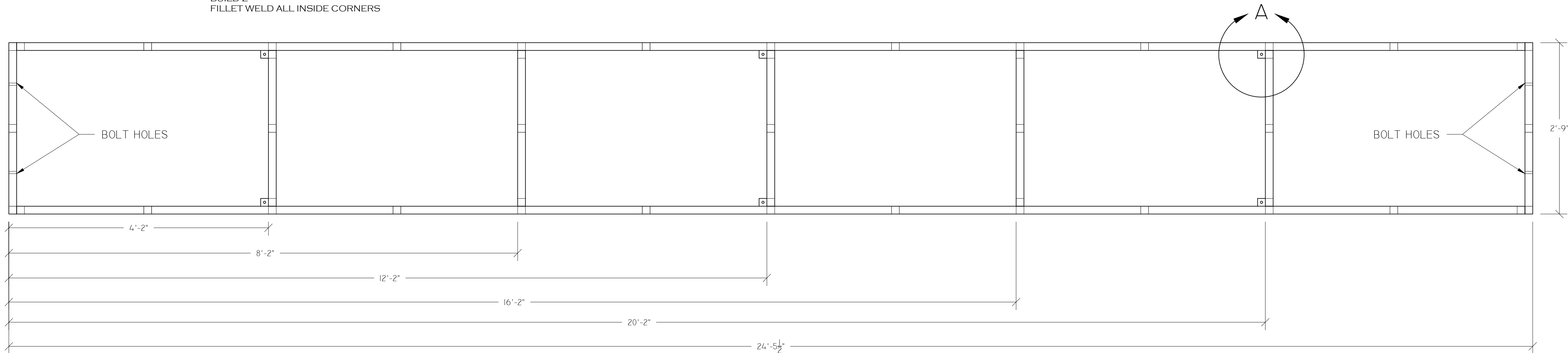
SECTION A+B PLAN VIEW BUILD 2 FILLET WELD ALL INSIDE CORNERS
