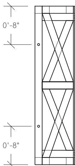
SECTION A+B SL VIEW DRILL 7/16" BOLT HOLES CENTERED ON BOX TUBING
