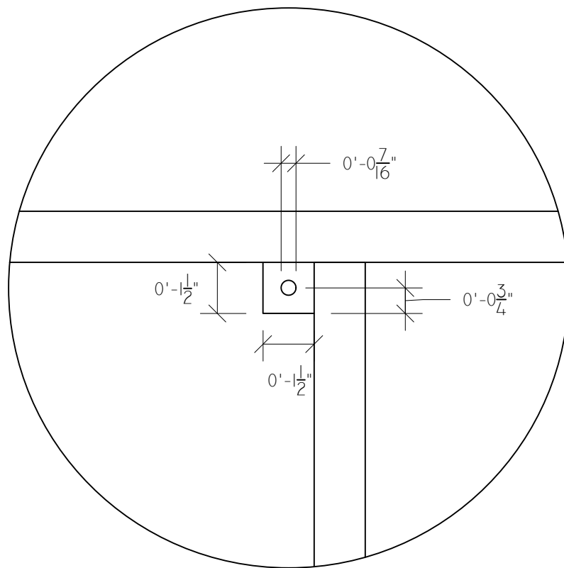
DETAIL A- CORNER TABS BUILD 32 USE 1/4"X1.5" FLAT BAR WELD INTO CORNER TO LAG FRAME INTO FLOOR
