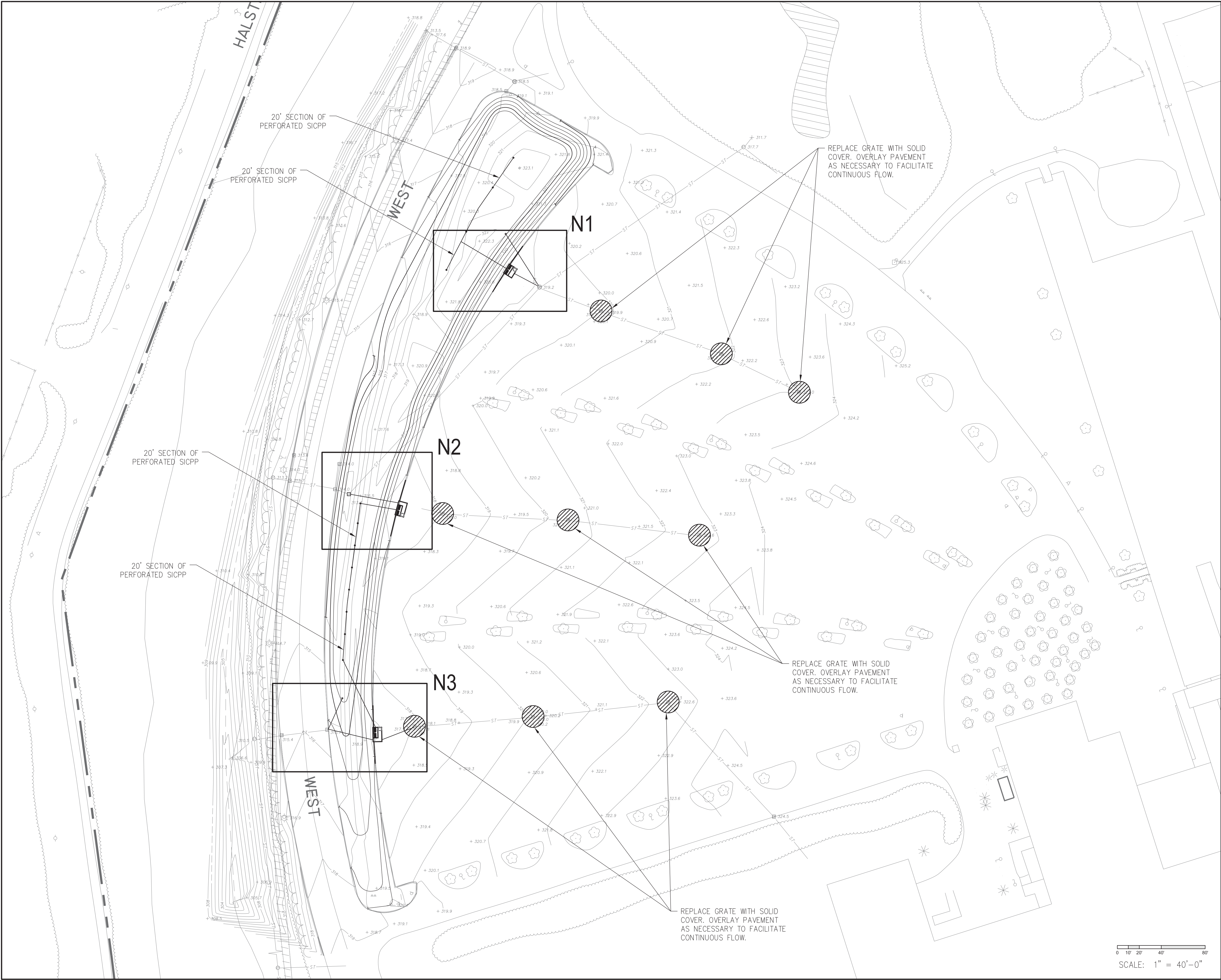
PROPOSED NORTH LOT PLAN SCALE: 1" = 40'-0"
