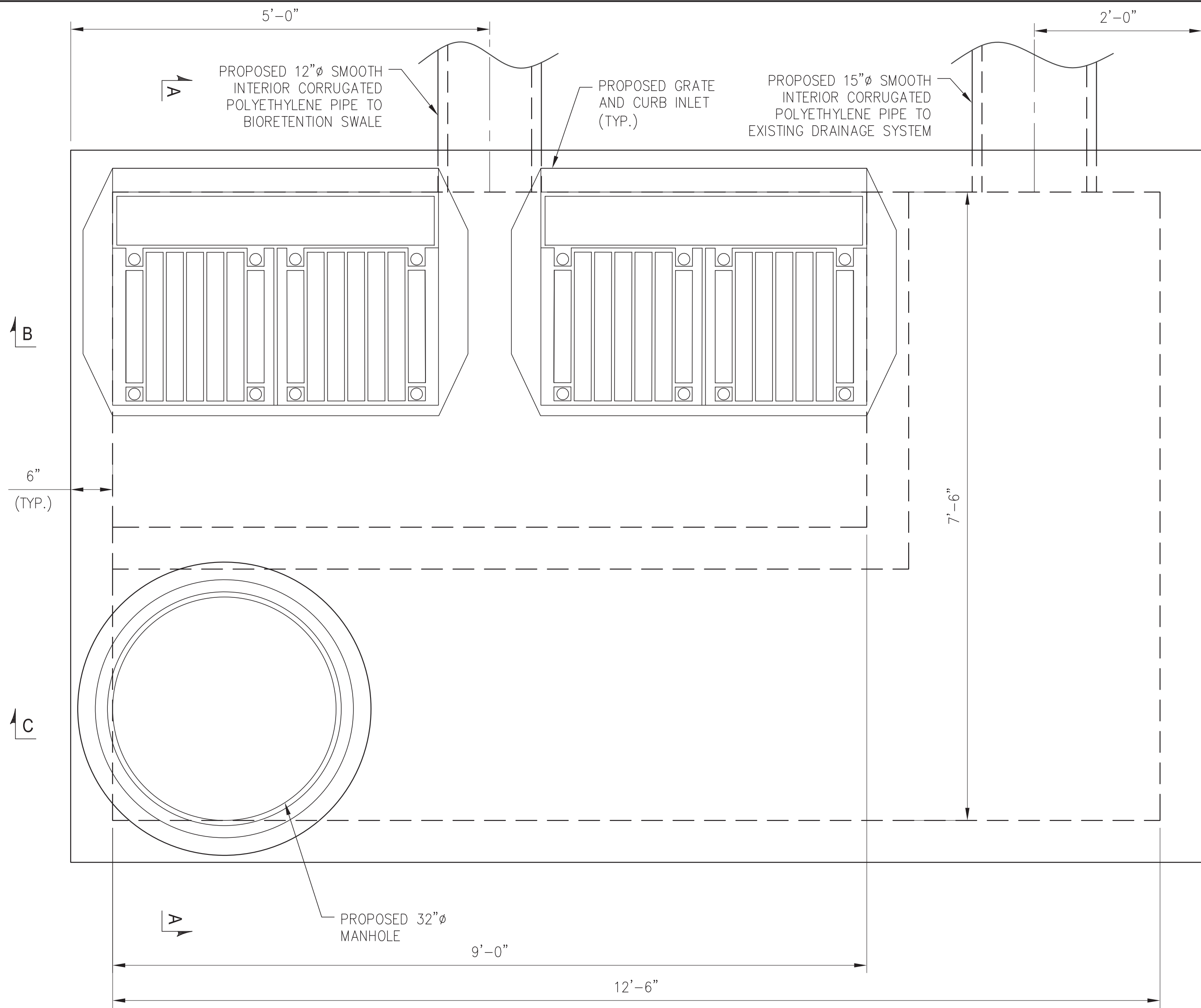
DRAINAGE STRUCTURE PLAN SCALE: 1" = 1'-0"
