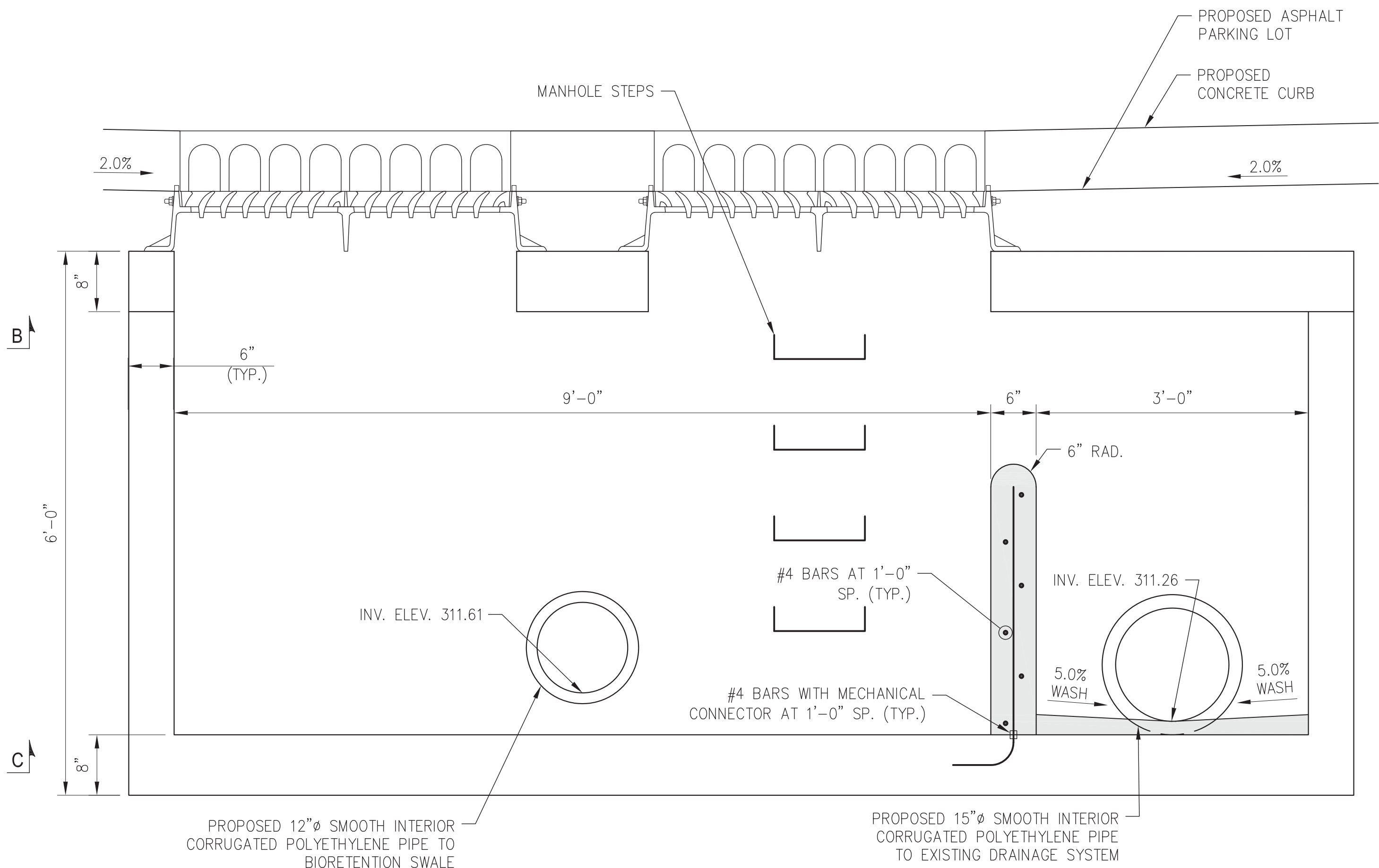
DRAINAGE STRUCTURE SECTION B-B SCALE: 1" = 1'-0"
