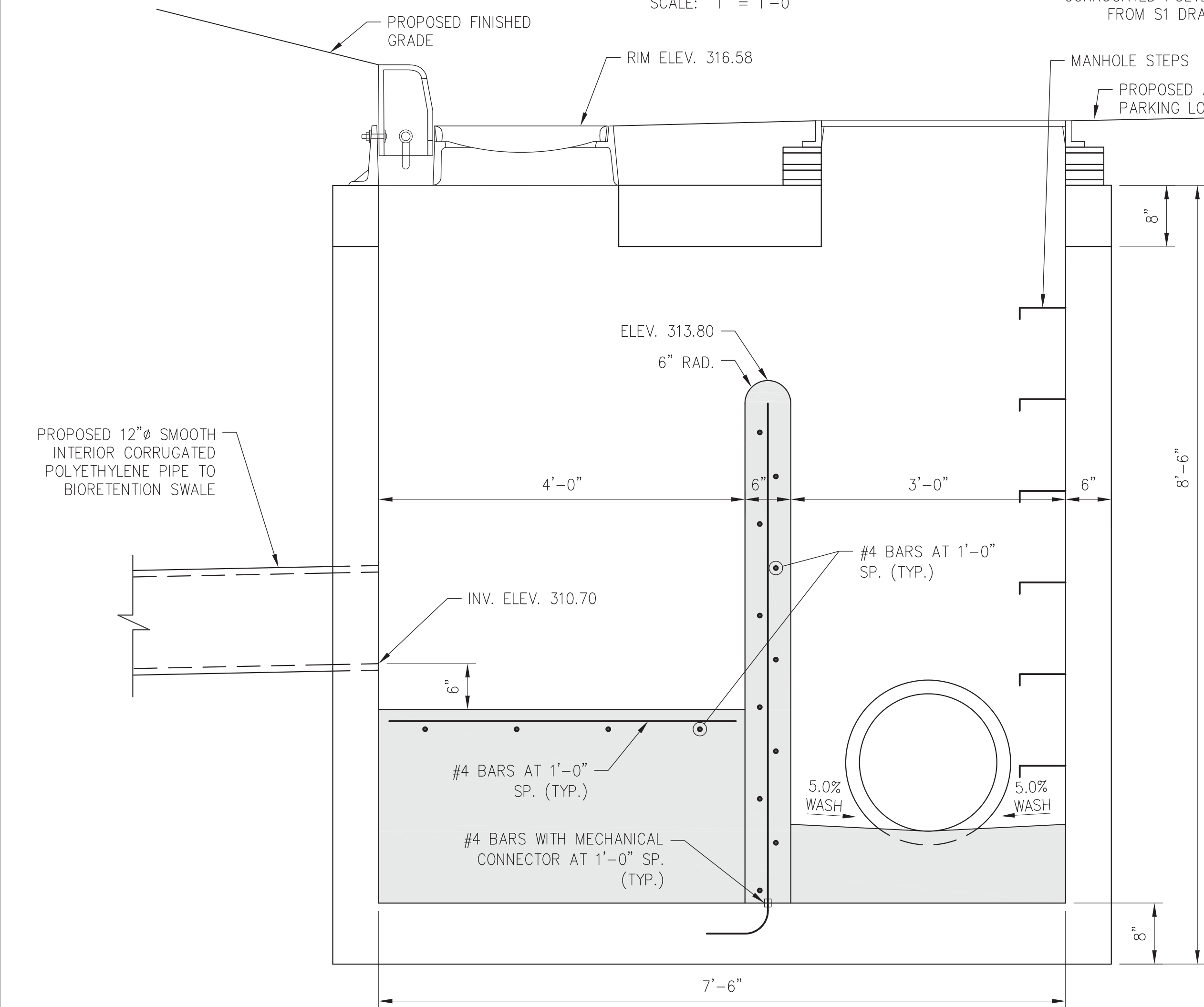
DRAINAGE STRUCTURE SECTION A-A
