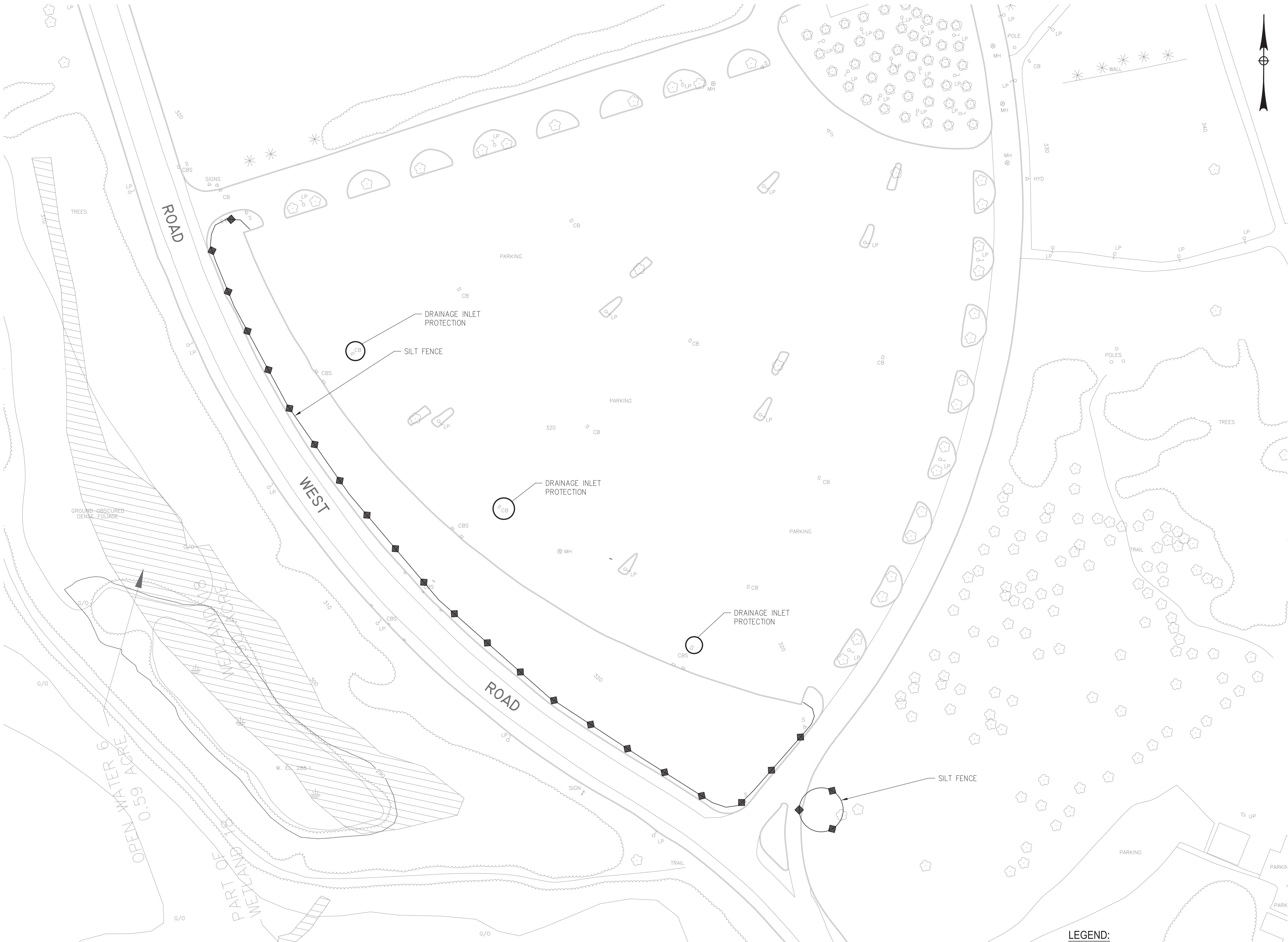
EROSION AND SEDIMENT CONTROL PLAN - SOUTH END SCALE: 1" = 40'-0"
