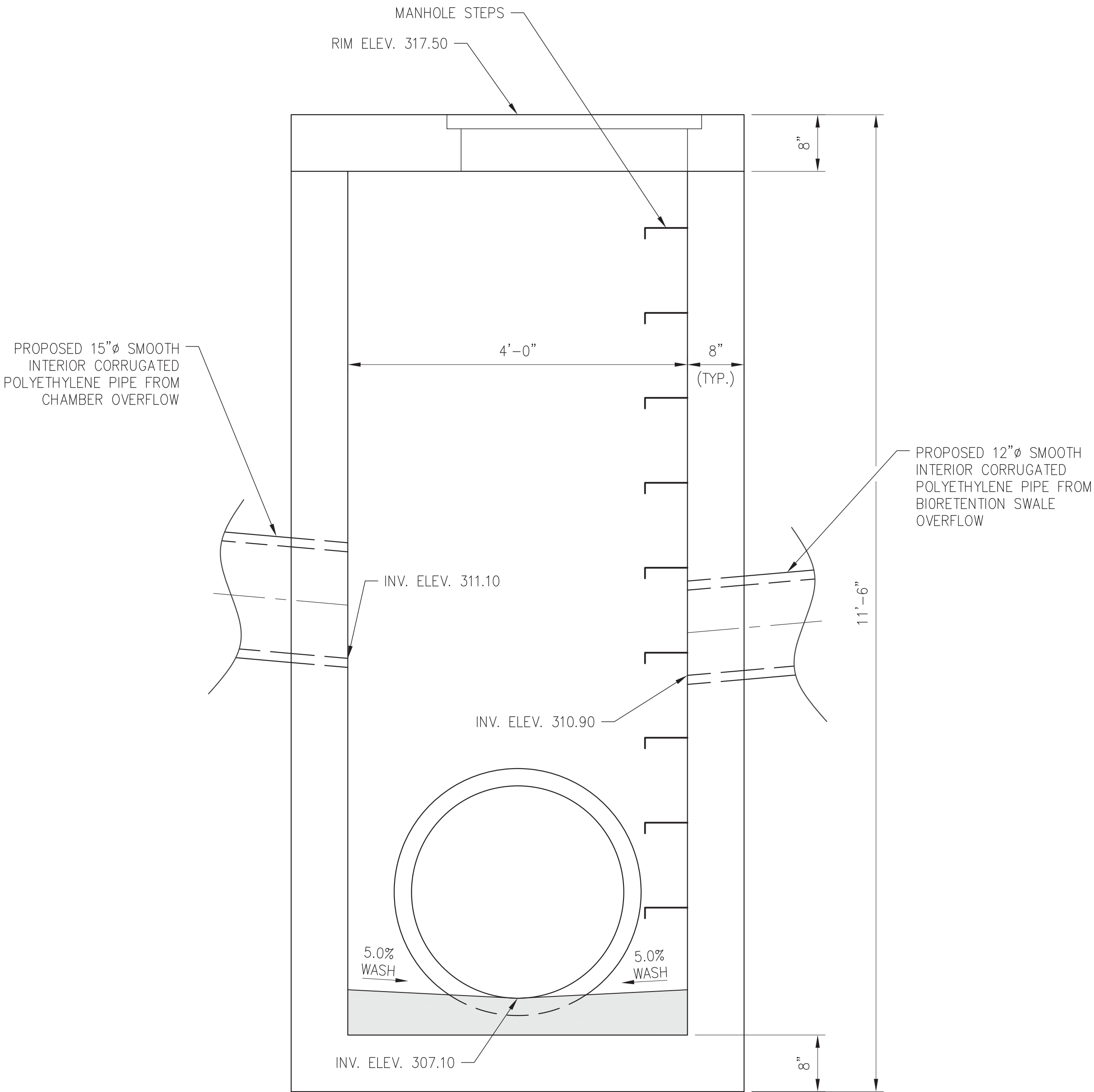
DRAINAGE STRUCTURE SECTION A-A SCALE: 1" = 1'-0"
