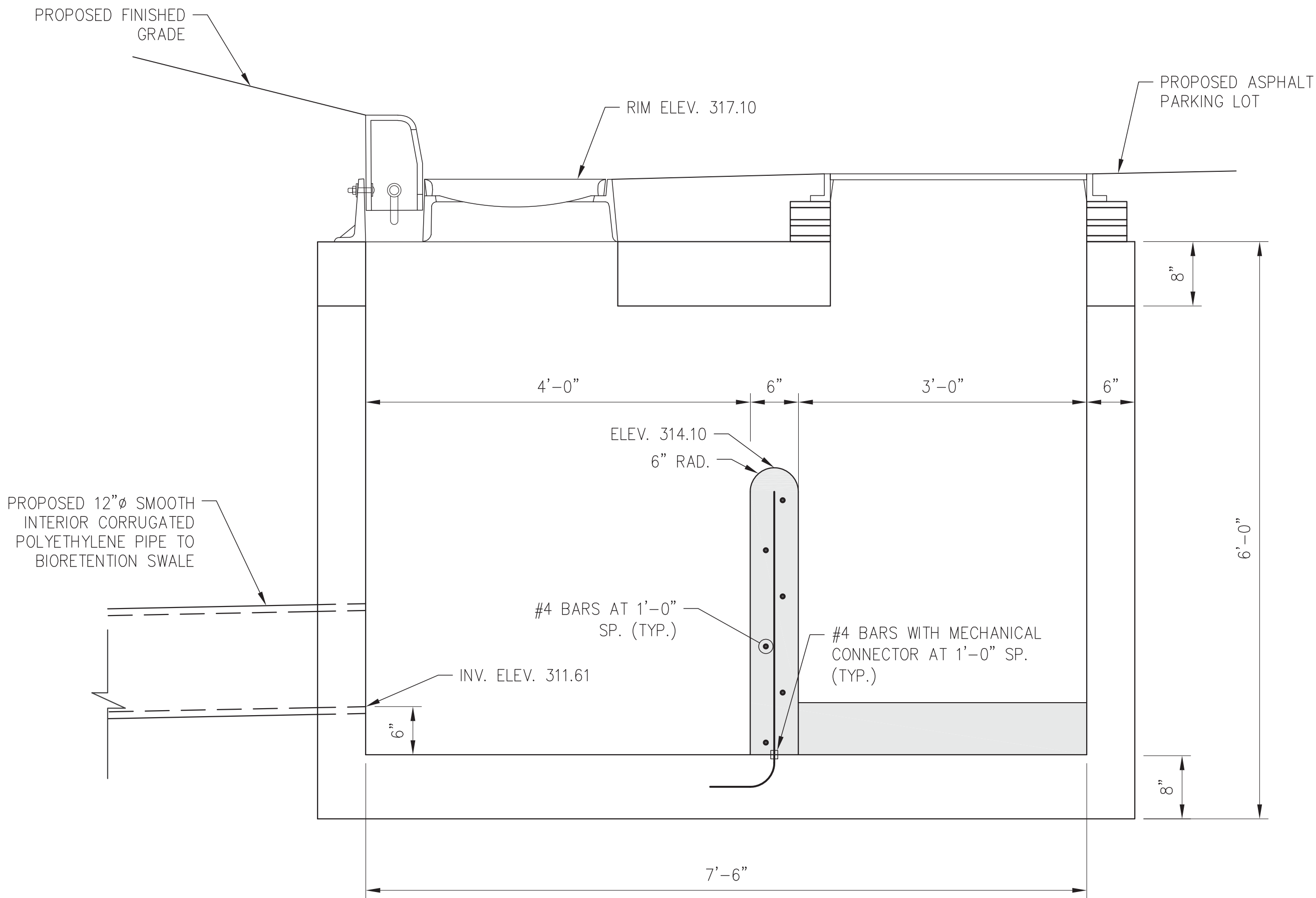
DRAINAGE STRUCTURE SECTION A-A SCALE: 1" = 1'-0"
