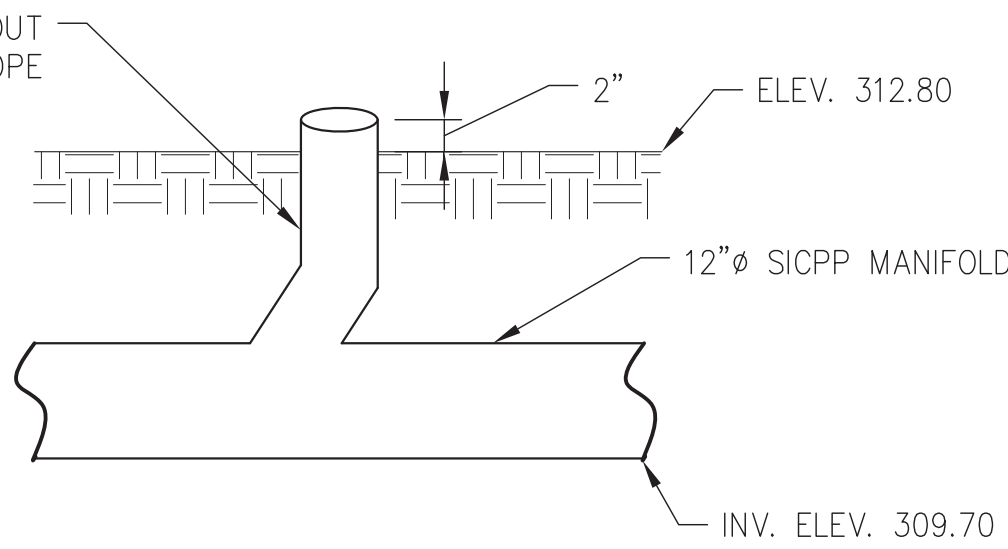
8" Ø UP SPOUT DETAIL NOT TO SCALE
