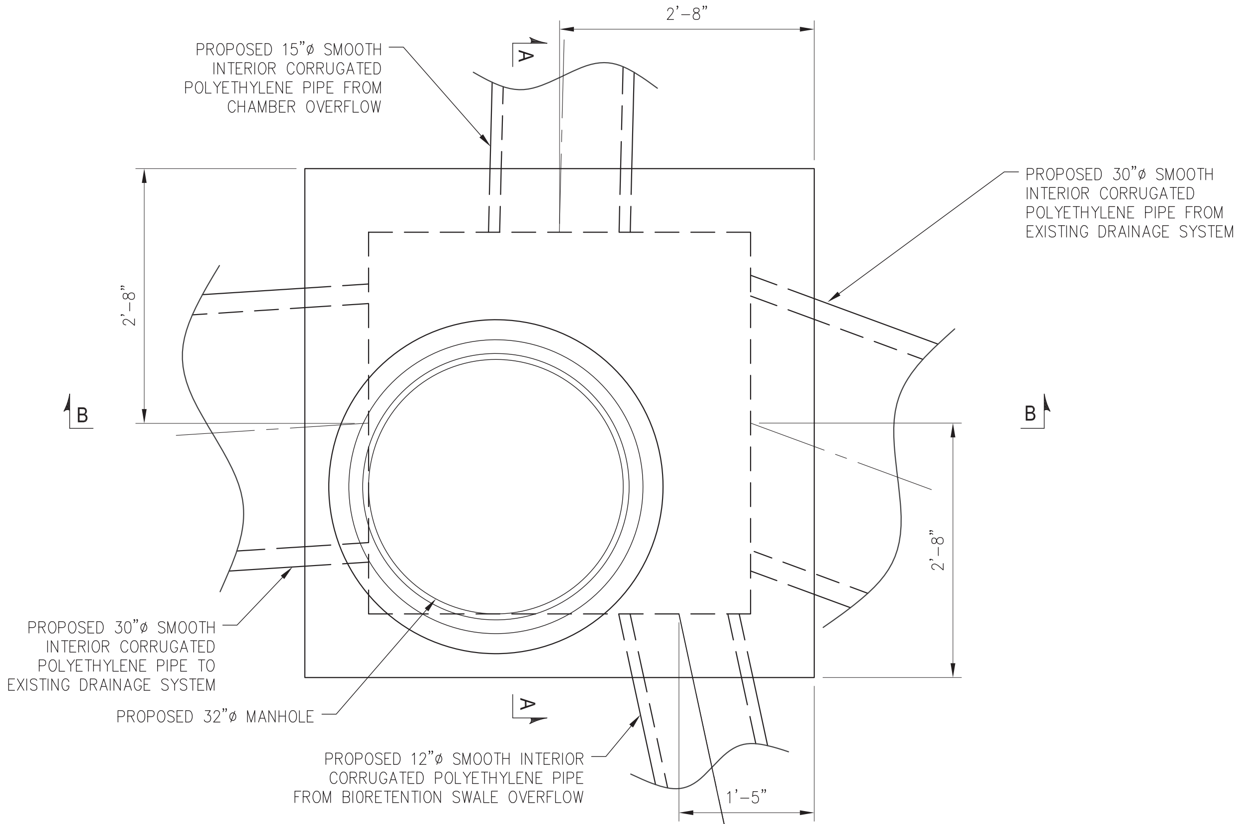
DRAINAGE STRUCTURE PLAN SCALE: 1" = 1'-0"
