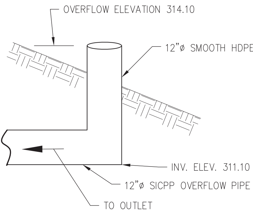
12" Ø BIORETENTION OVERFLOW DETAIL NOT TO SCALE
