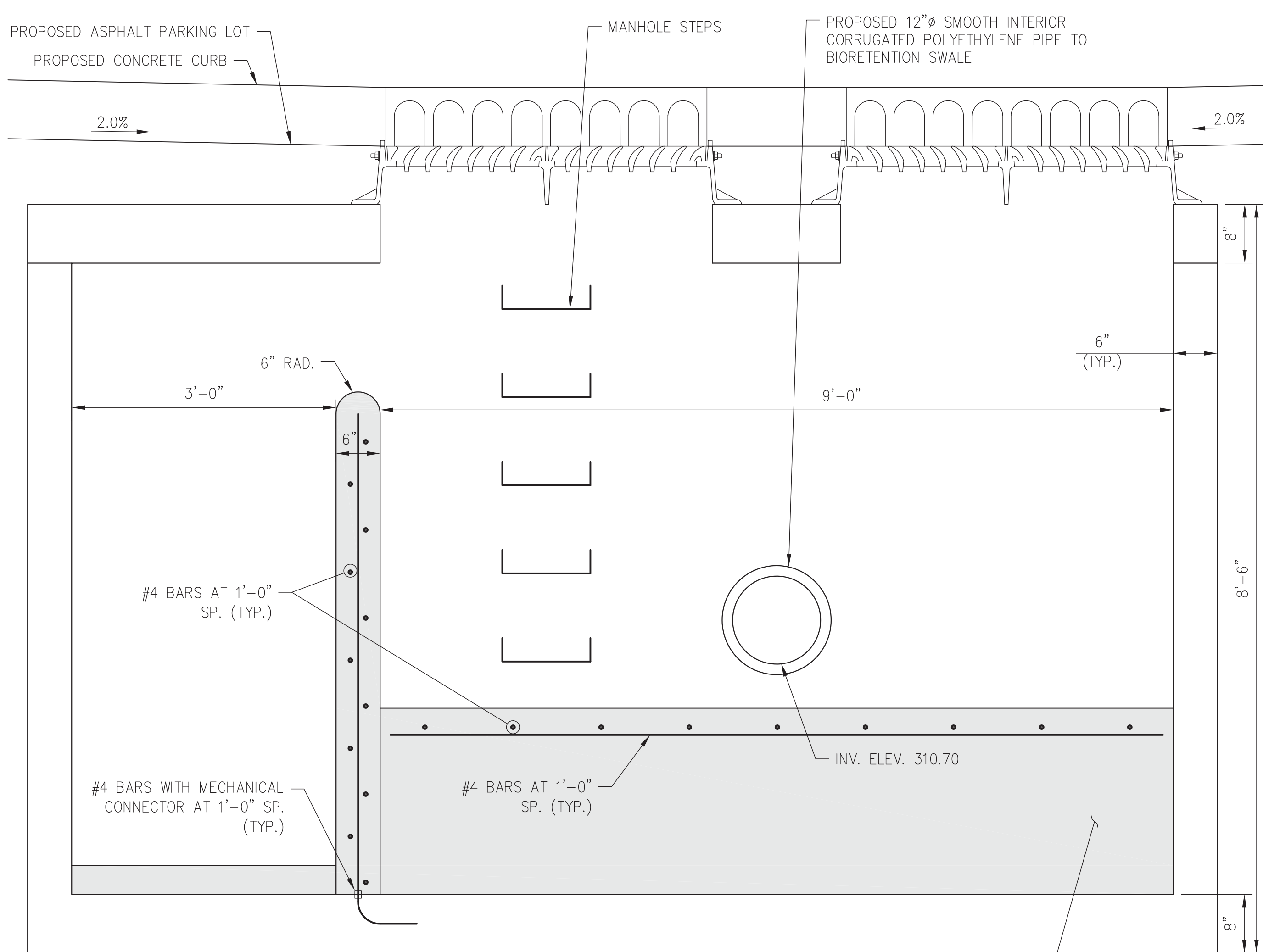
DRAINAGE STRUCTURE SECTION B-B
