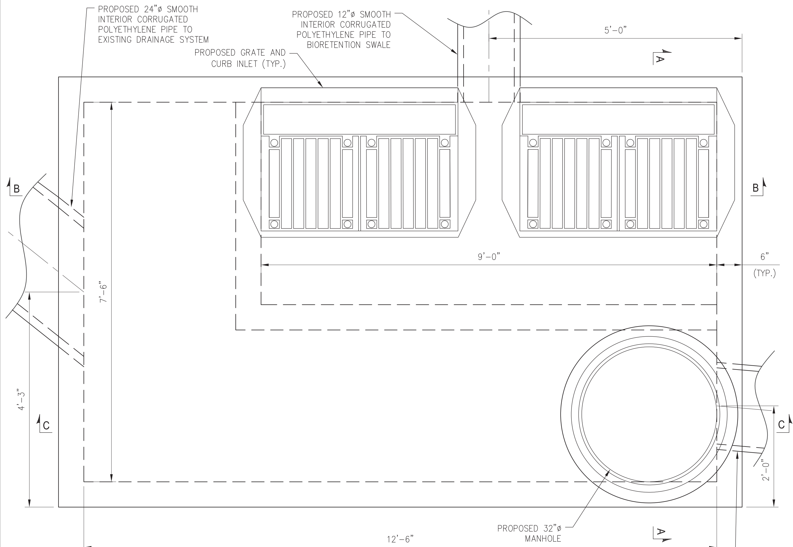
DRAINAGE STRUCTURE PLAN
