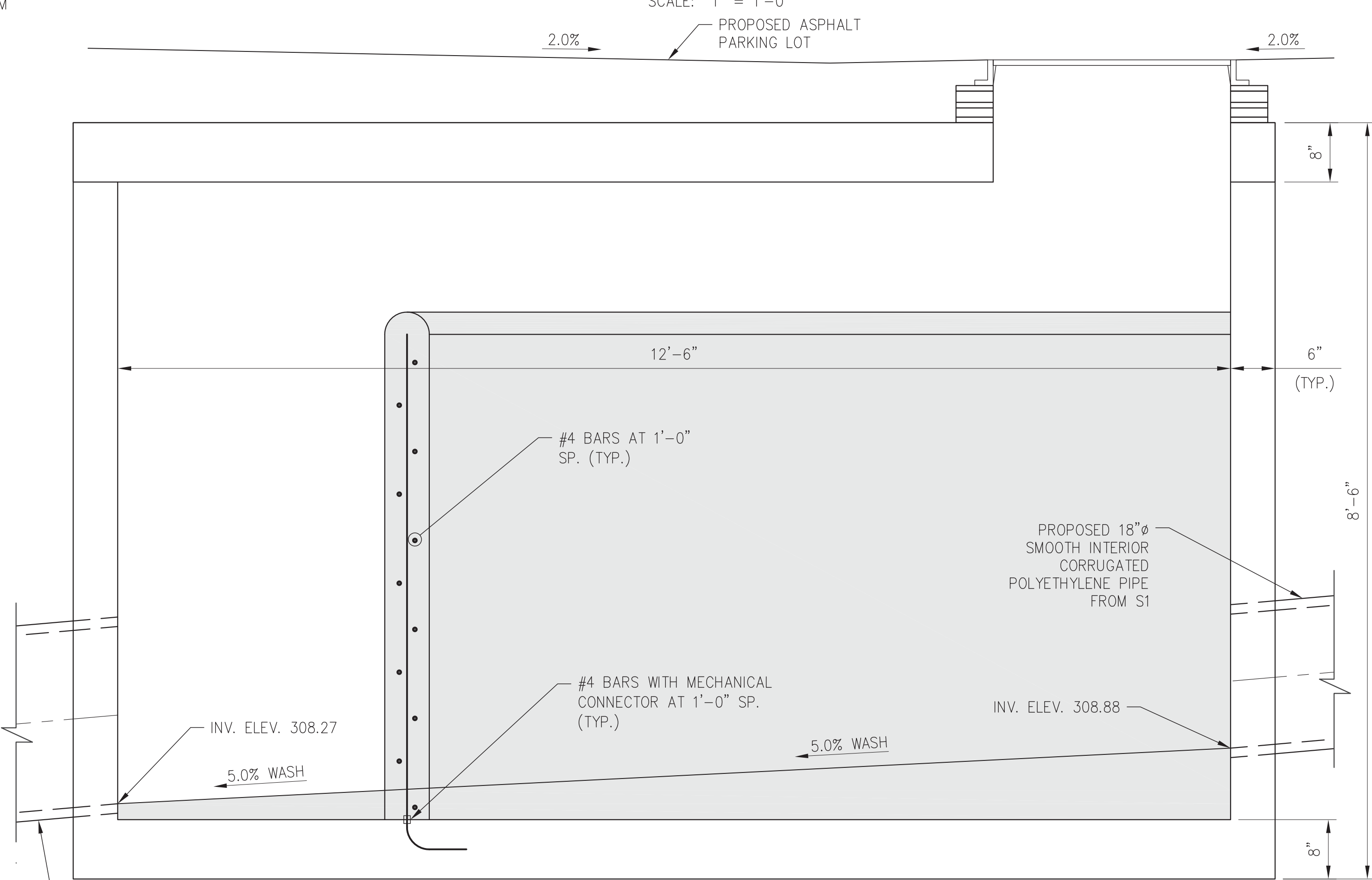
DRAINAGE STRUCTURE SECTION C-C
