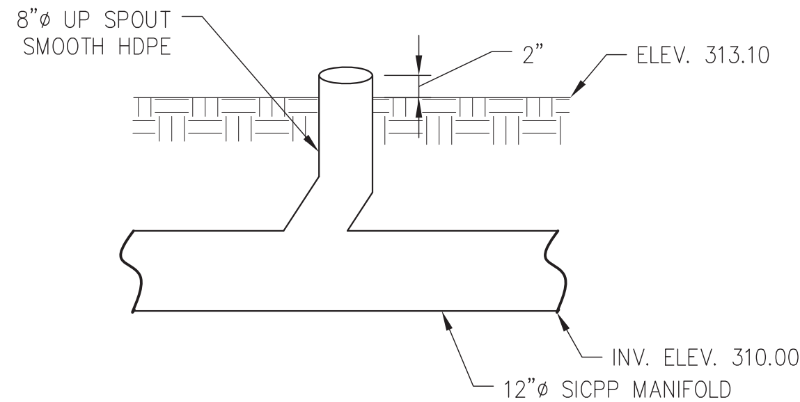
8" Ø UP SPOUT DETAIL NOT TO SCALE
