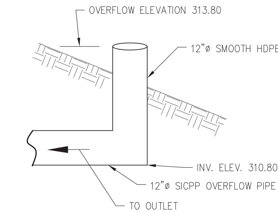
12" Ø BIORETENTION OVERFLOW DETAIL NOT TO SCALE
