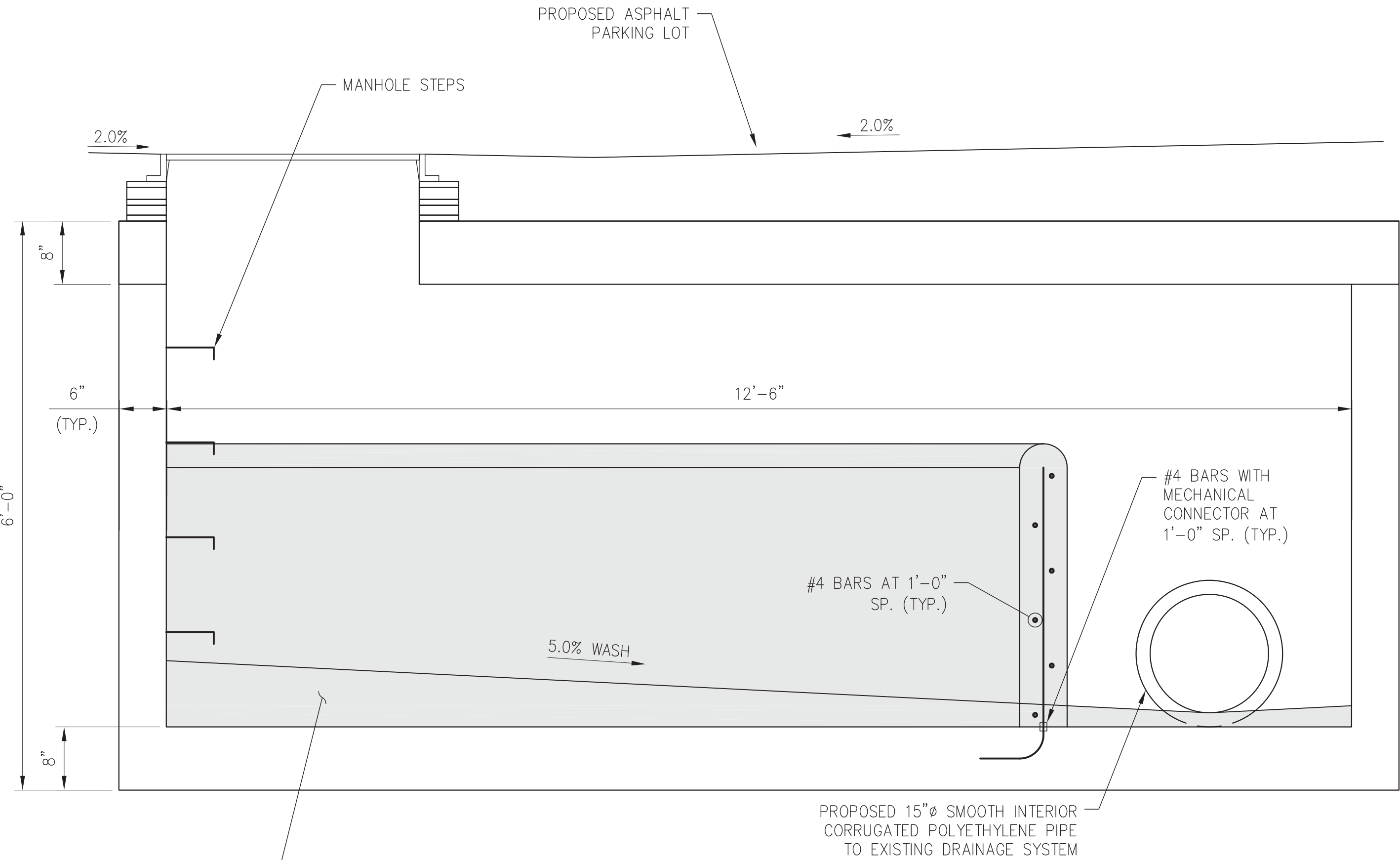
DRAINAGE STRUCTURE SECTION C-C SCALE: 1" = 1'-0"
