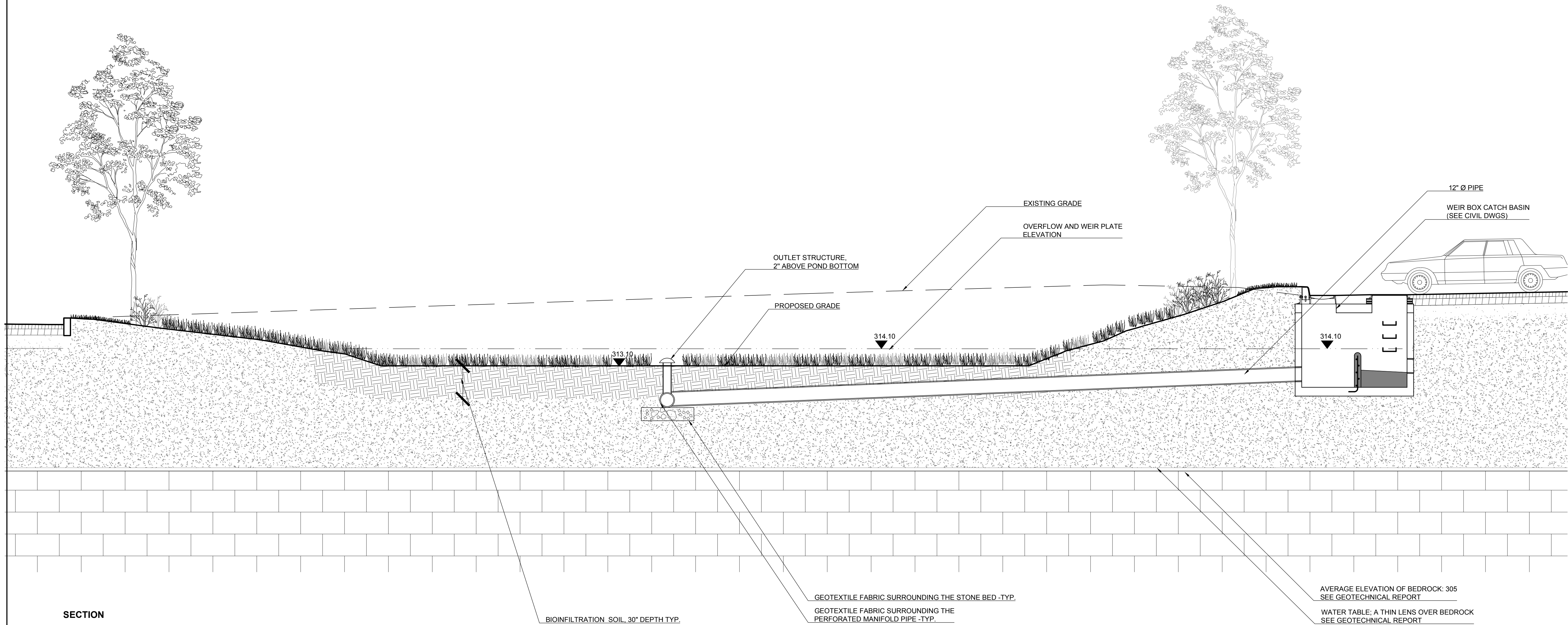
SECTION 1 LM-302 1/4"=1'-0" INFILTRATING BIORETENTION BASIN N1
