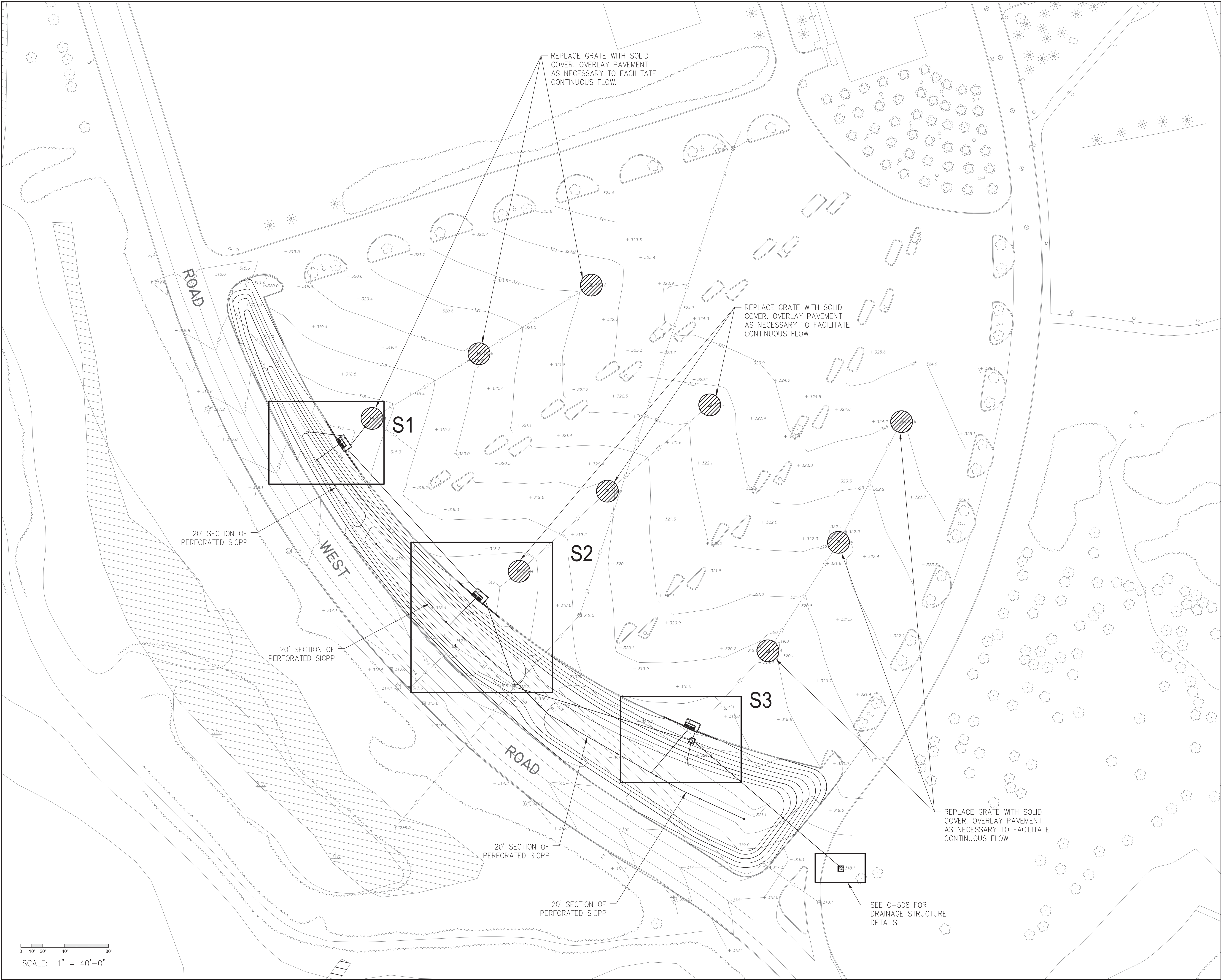
PROPOSED SOUTH LOT PLAN SCALE: 1" = 40'-0"
