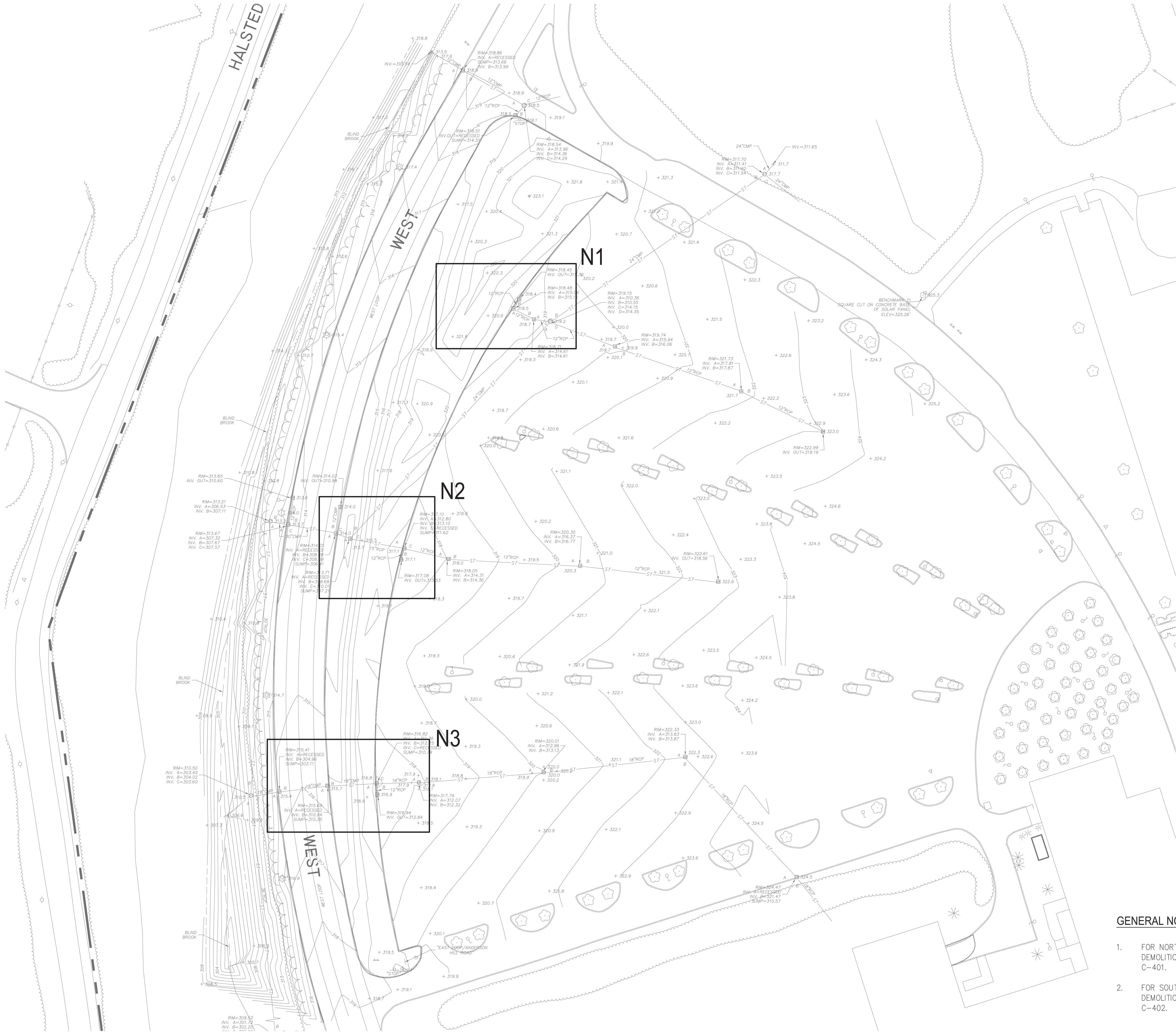
GENERAL NORTH LOT PLAN SCALE: 1" = 40'-0"
