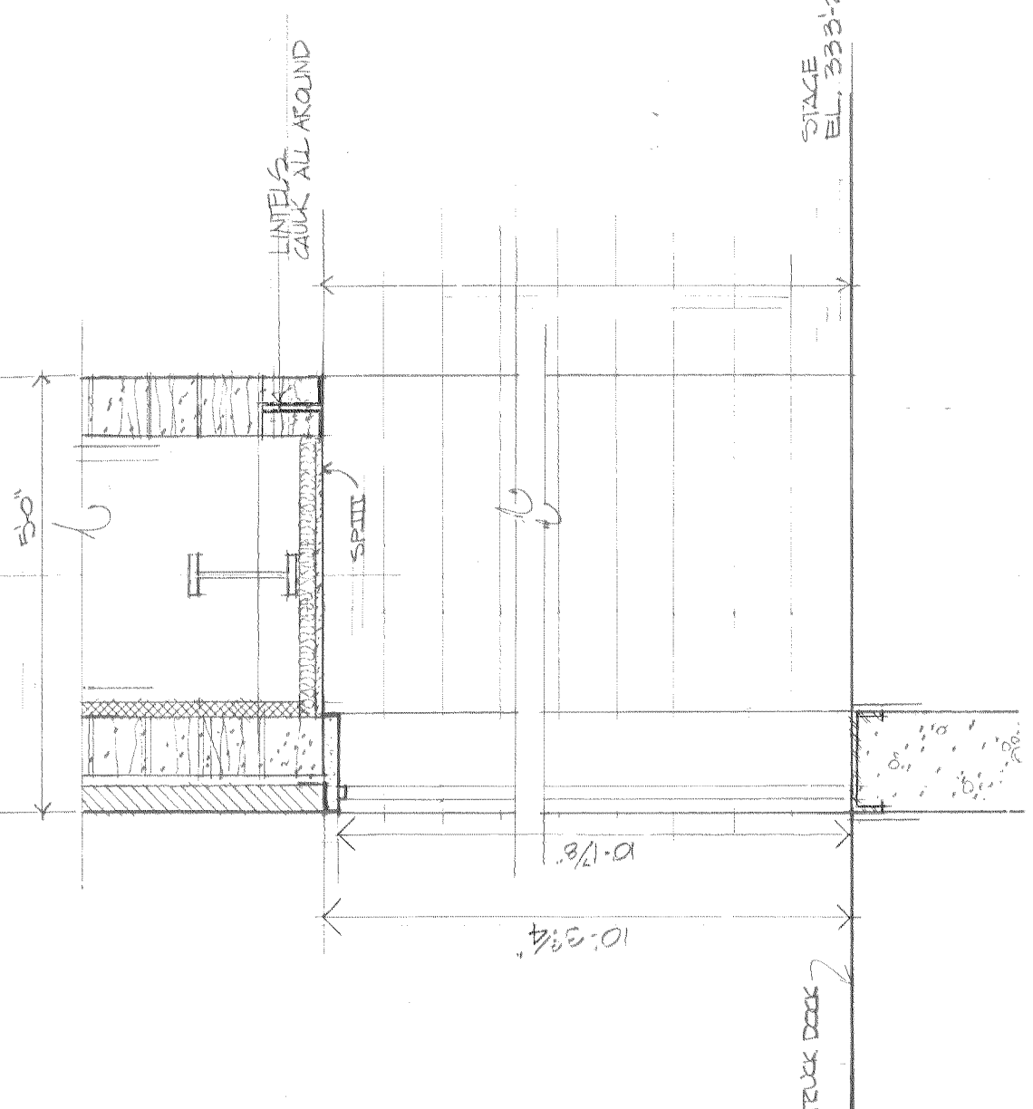
SECTION C TRUCK DOCK DOOR SCALE: 1/2" = 1'-0"
